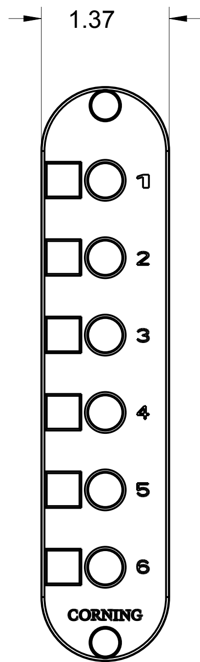
FRONT
