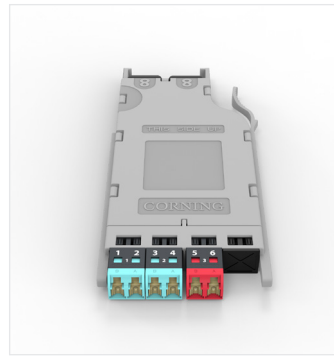
EDGE8 LC to LC Tap Module Photo REN3237
