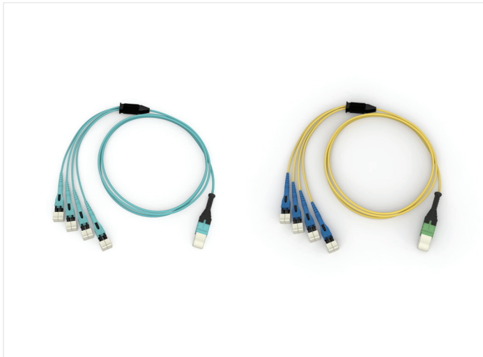
EDGE8 Staggered Harness MM and SM | Photos REN7930 and REN7959
