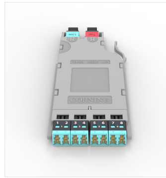
EDGE8 MTP to LC Duplex Tap Module Photo REN3222
