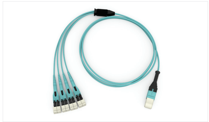
EDGE8 Non-Staggered Harness | Photo REN7931
