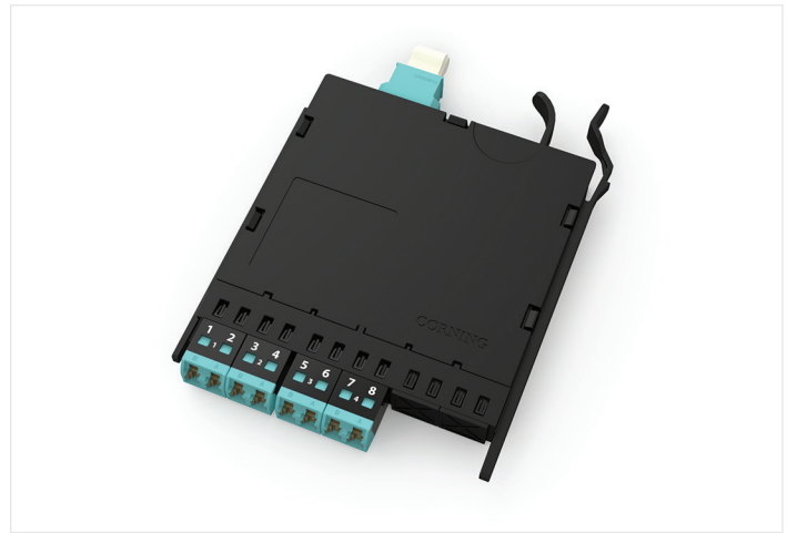
EDGE Base-8 MTP to LC Duplex Module | Photo REN6520
