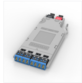
EDGE8 MTP to LC Duplex Tap Module Photo REN3252
